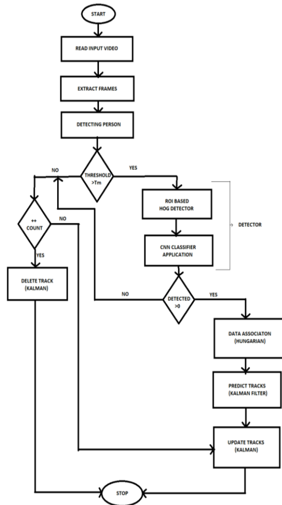
Figure 3: Flow Chart of CNN Classifier with ROI Based HOG Detection Results
